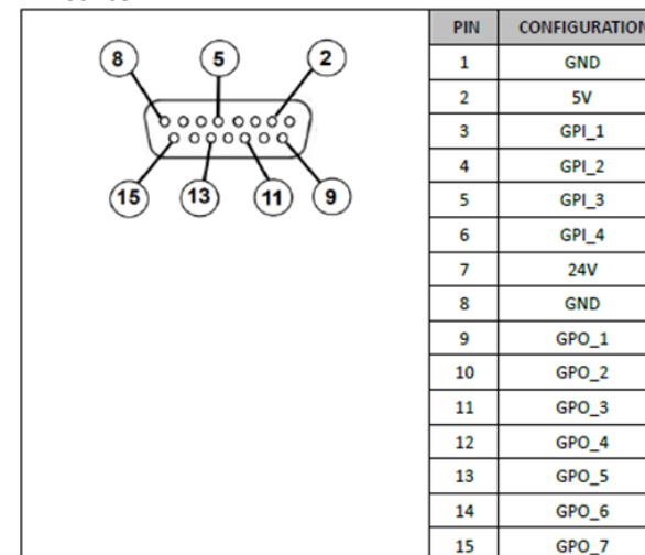
MB series
