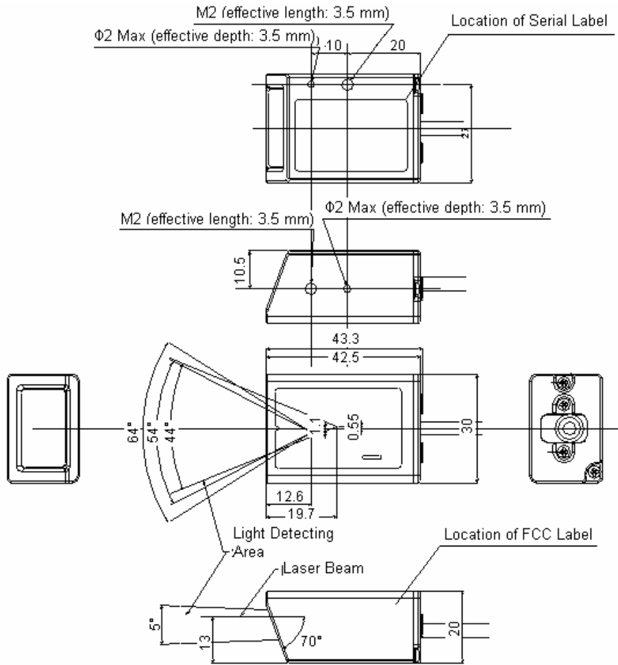
Figure 33: Mechanical drawing
